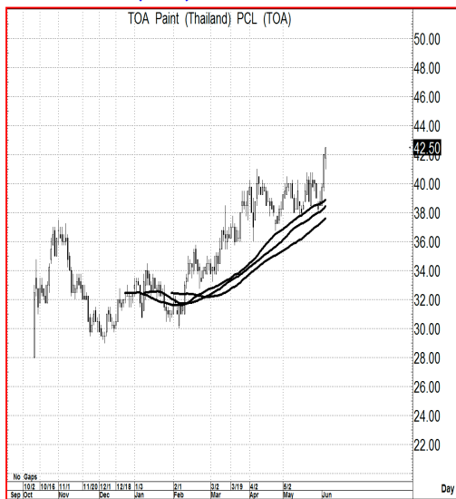
Price Chart...(TOA)
